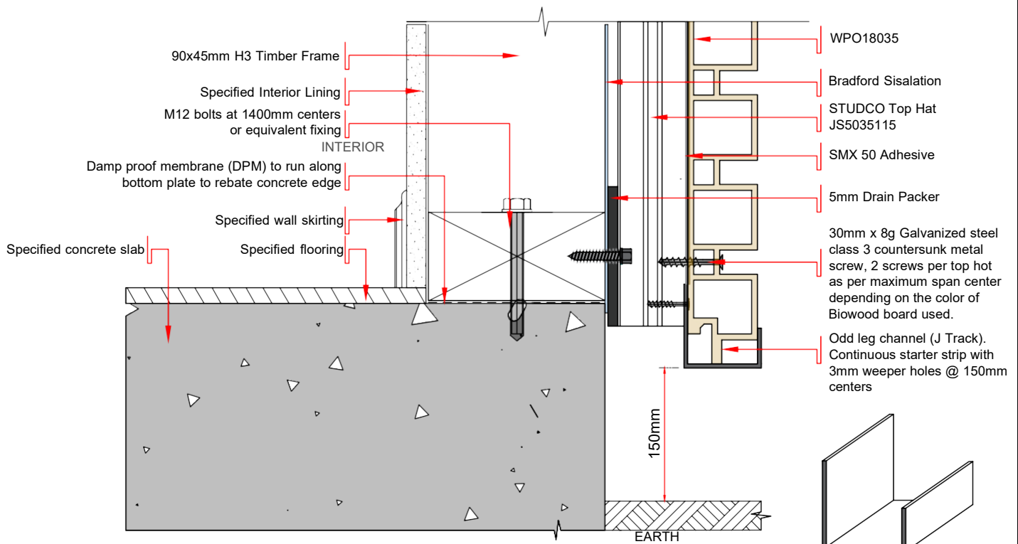
DWG - 03 SECTION VIEW OF CONCRETE EDGE SLAB EDGE DETAIL OF HORIZONTAL LAID BIOWOOD CLADDING - WPO18035 SCALE 1:2.5 @ A4
