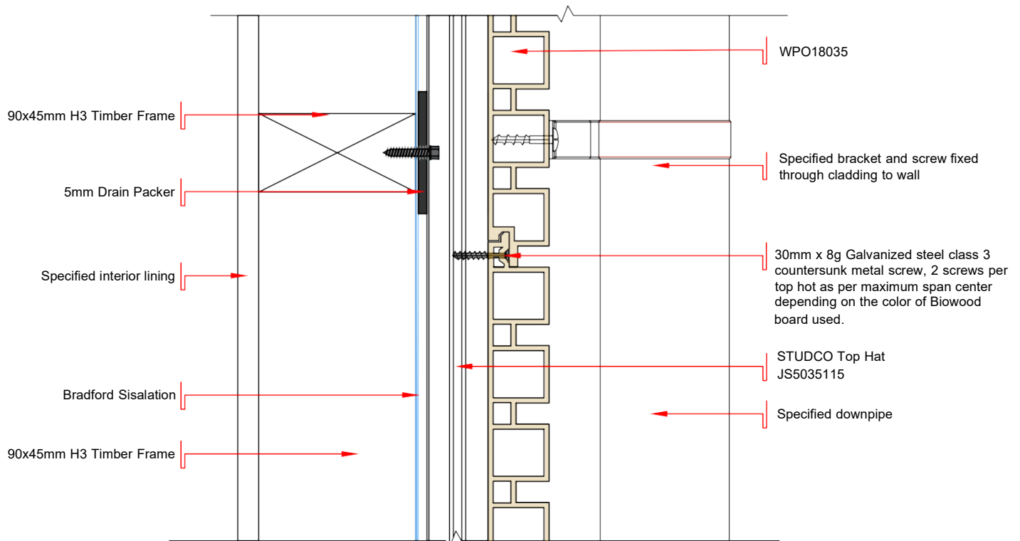
DWG - 13 SECTION VIEW OF DOWNPIPE FIXING DETAIL OF HORIZONTAL LAID BIOWOOD CLADDING - WPO18035 SCALE 1:3 @ A4
