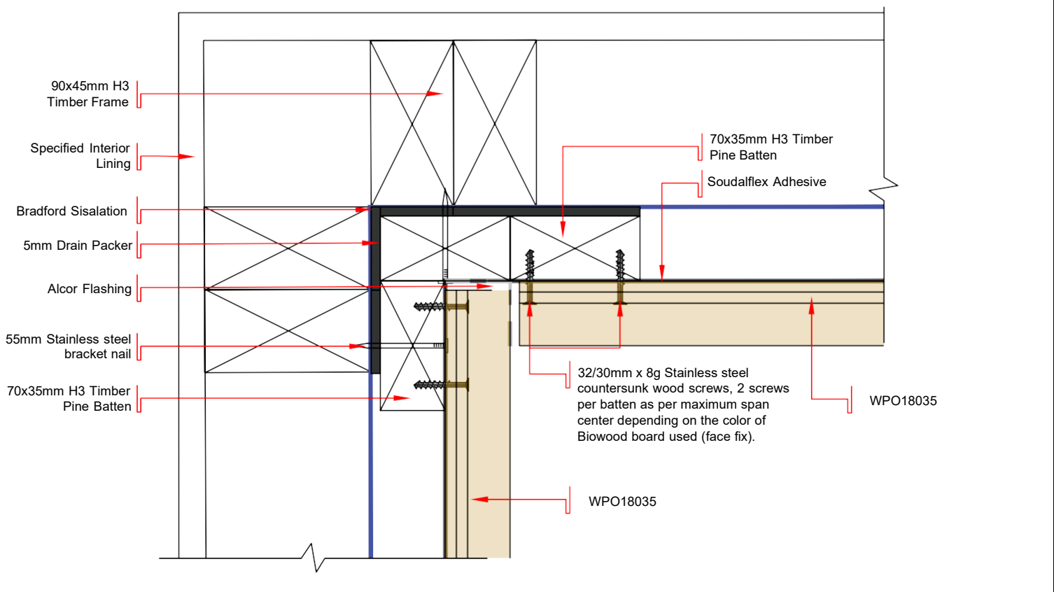
DWG - 05 PLAN VIEW OF INTERNAL CORNER DETAIL OF HORIZONTAL LAID BIOWOOD CLADDING - WPO18035 SCALE 1:3 @ A4
