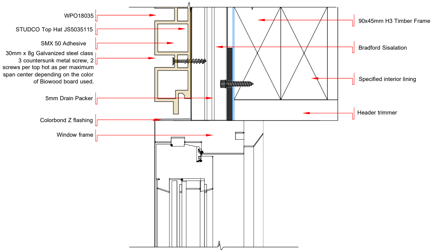
DWG - 06 SECTION VIEW OF WINDOW HEAD DETAIL OF HORIZONTAL LAID BIOWOOD CLADDING - WPO18035 SCALE 1:2.2 @ A4
