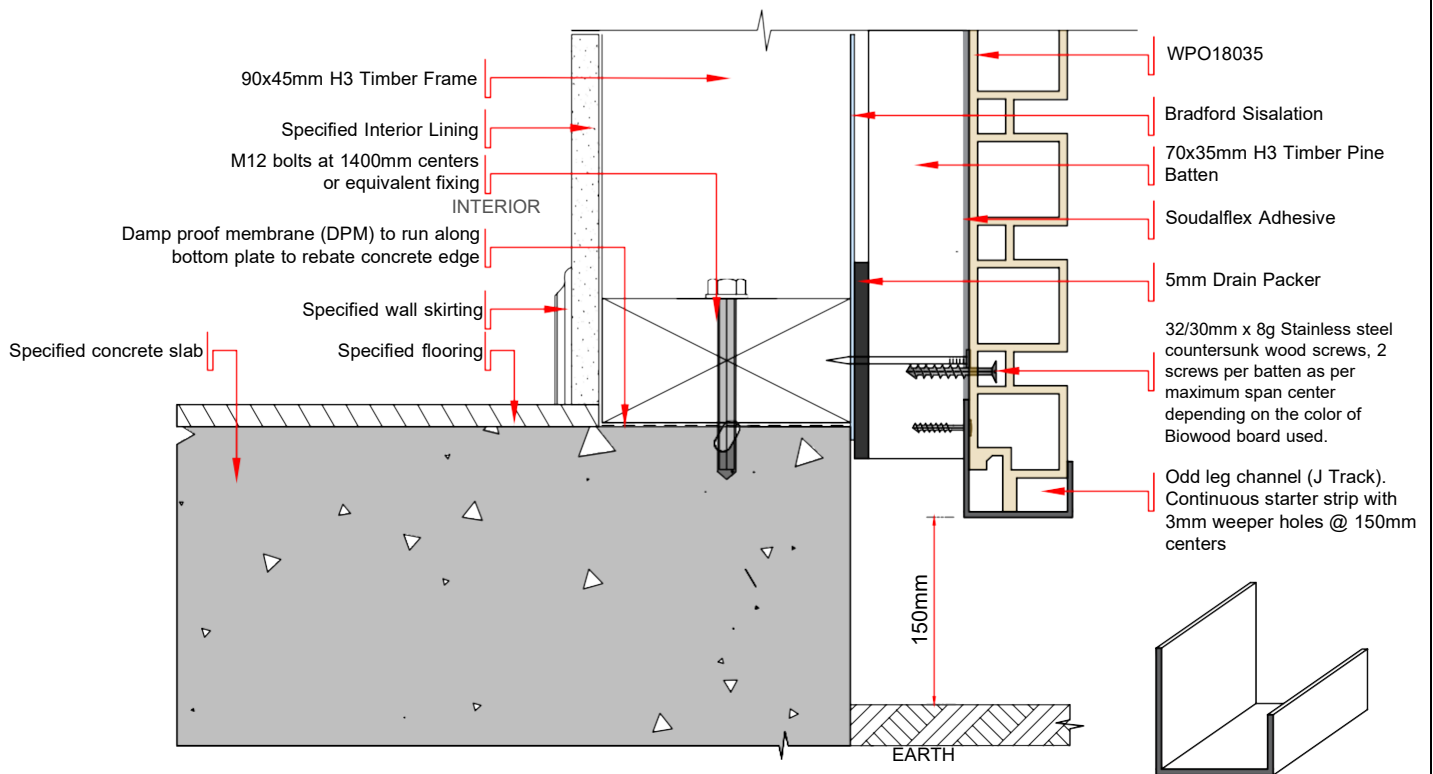
DWG - 03 SECTION VIEW OF CONCRETE EDGE SLAB EDGE DETAIL OF HORIZONTAL LAID BIOWOOD CLADDING - WPO18035 SCALE 1:2.5 @ A4
