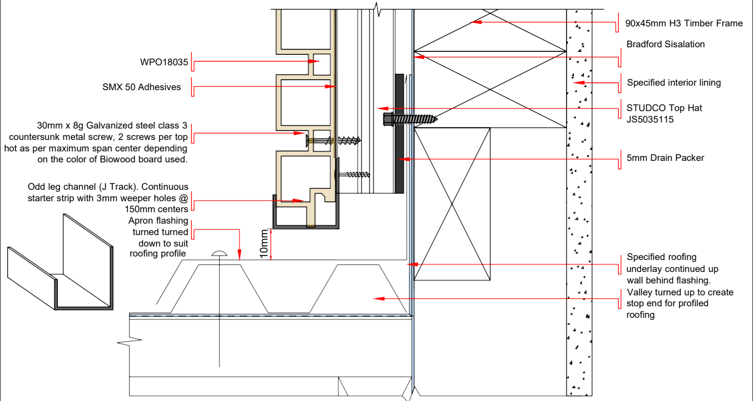
DWG - 10 SECTION VIEW OF PARALLEL APRON DETAIL OF HORIZONTAL LAID BIOWOOD CLADDING - WPO18035 SCALE 1:2.2 @ A4
