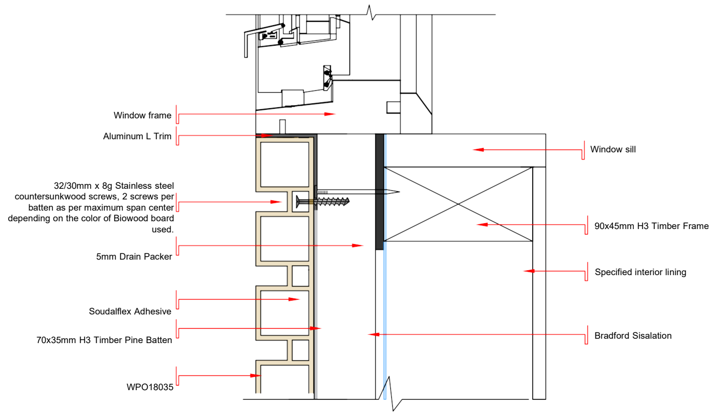
DWG - 07 SECTION VIEW OF WINDOW SILL DETAIL OF HORIZONTAL LAID BIOWOOD CLADDING - WPO18035 SCALE 1:2.2 @ A4
