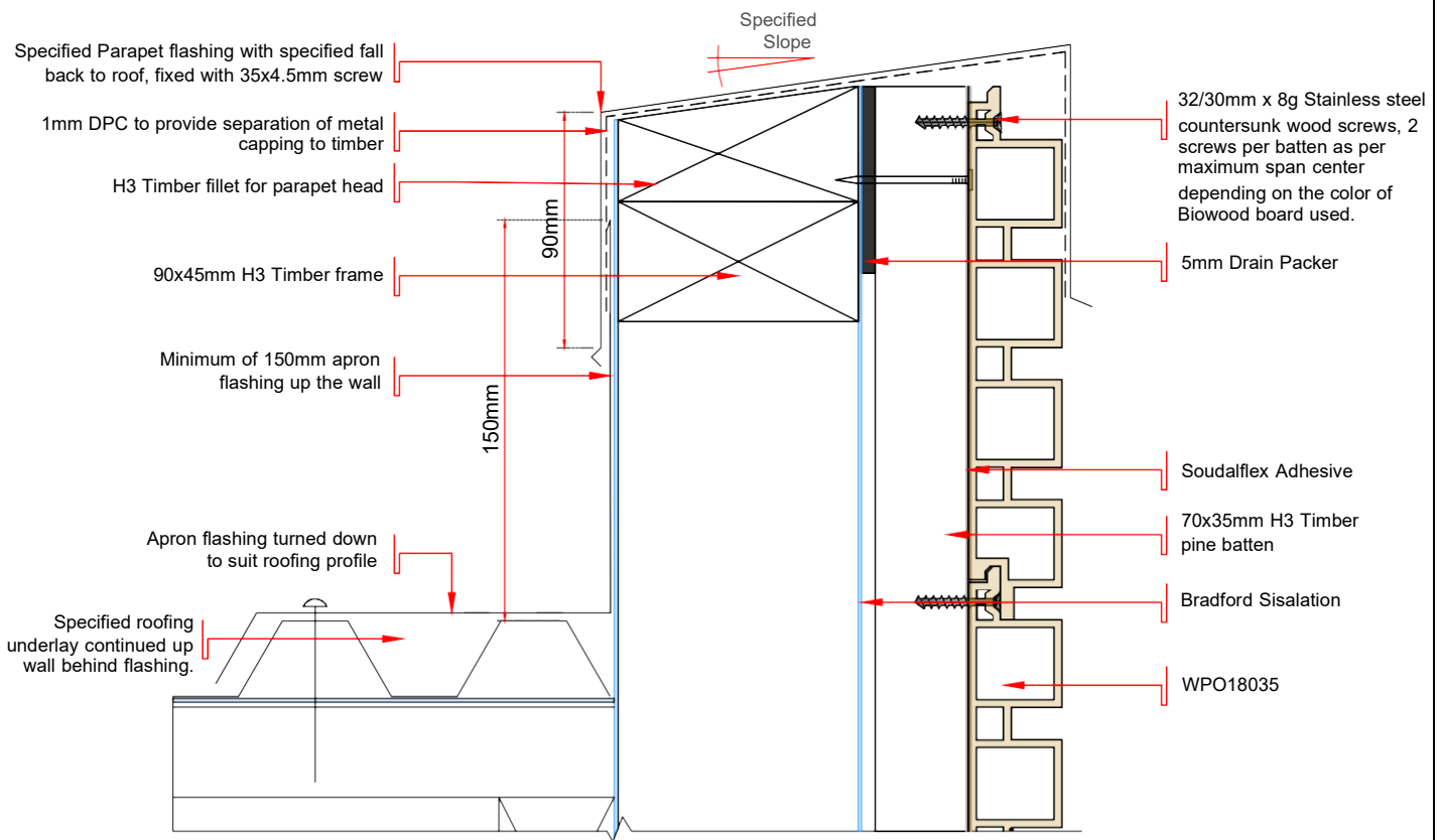
DWG - 12 SECTION VIEW OF PARAPET TO ROOF JUNCTION DETAIL OF HORIZONTAL LAID BIOWOOD CLADDING - WPO18035 SCALE 1:3 @ A4
