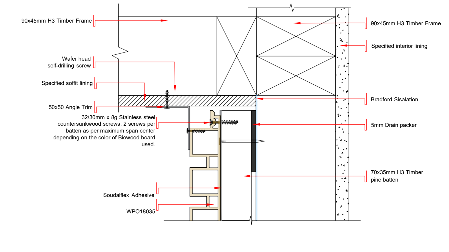
DWG - 11 SECTION VIEW OF CLADDING TO SOFFIT DETAIL OF HORIZONTAL LAID BIOWOOD CLADDING - WPO18035 SCALE 1:2.5 @ A4
