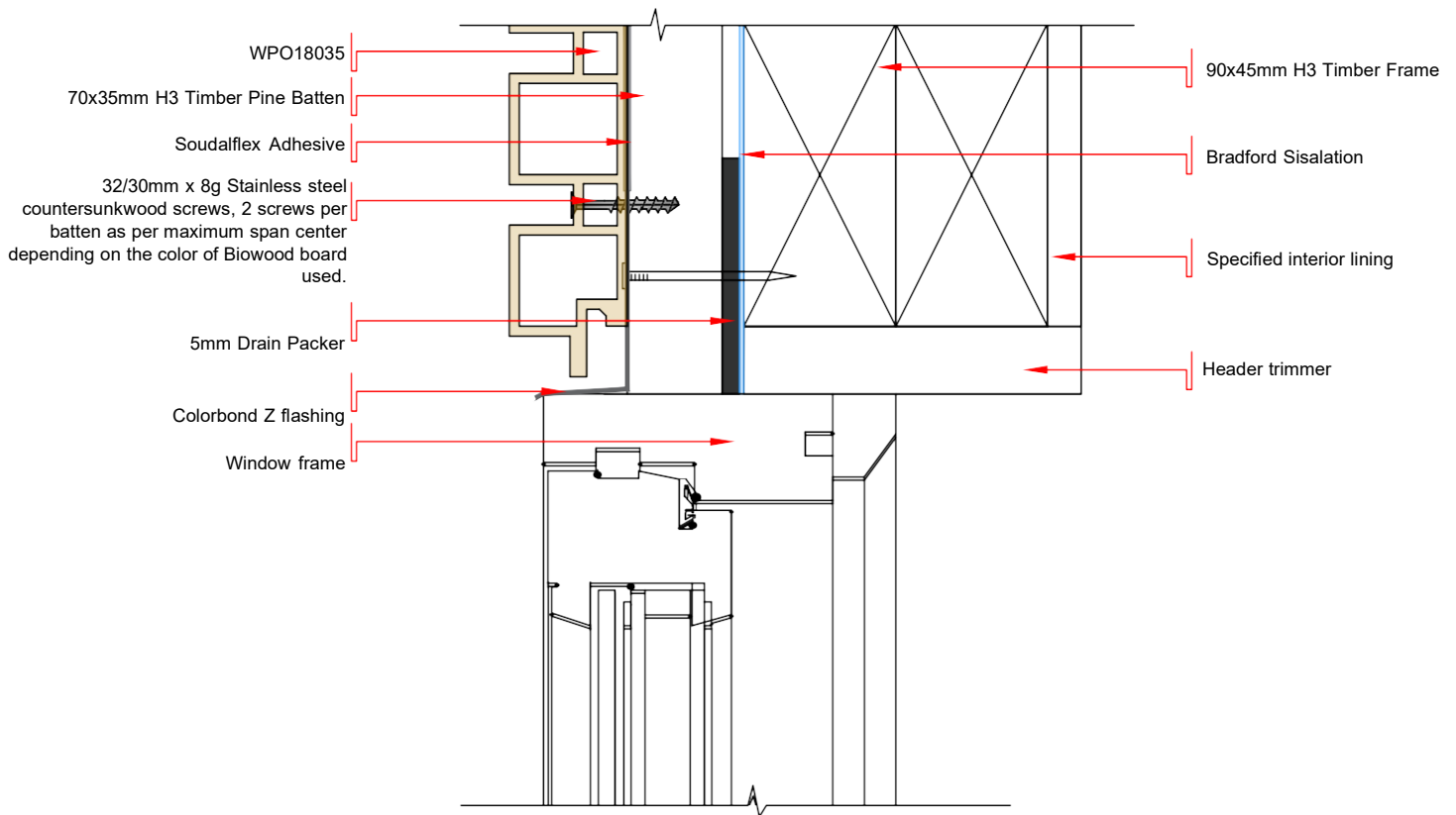
DWG - 06 SECTION VIEW OF WINDOW HEAD DETAIL OF HORIZONTAL LAID BIOWOOD CLADDING - WPO18035 SCALE 1:2.2 @ A4
