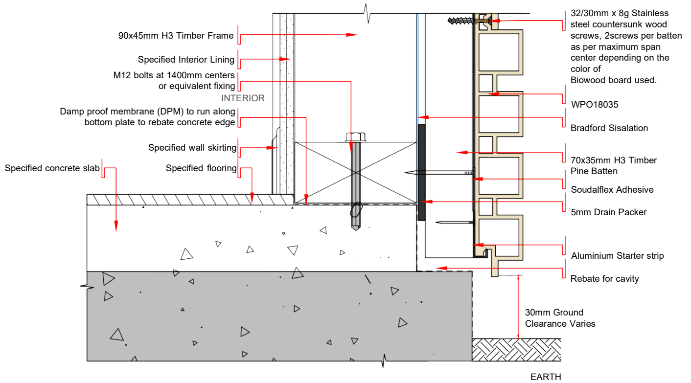
DWG - 02 SECTION VIEW OF REBATED EDGE SLAB EDGE DETAIL OF HORIZONTAL LAID BIOWOOD CLADDING - WPO18035 SCALE 1:2.5 @ A4
