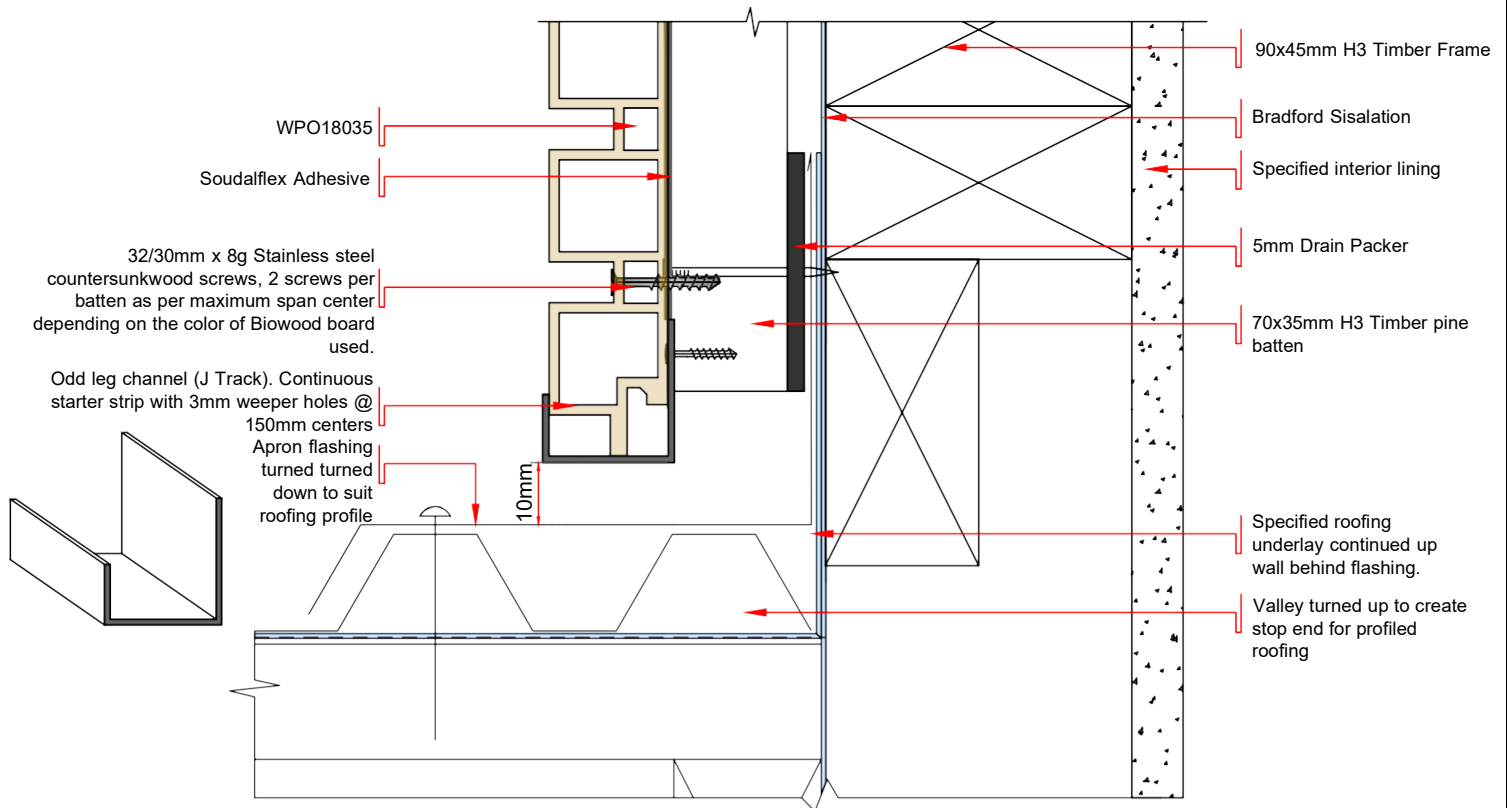
DWG - 10 SECTION VIEW OF PARALLEL APRON DETAIL OF HORIZONTAL LAID BIOWOOD CLADDING - WPO18035 SCALE 1:2.2 @ A4
