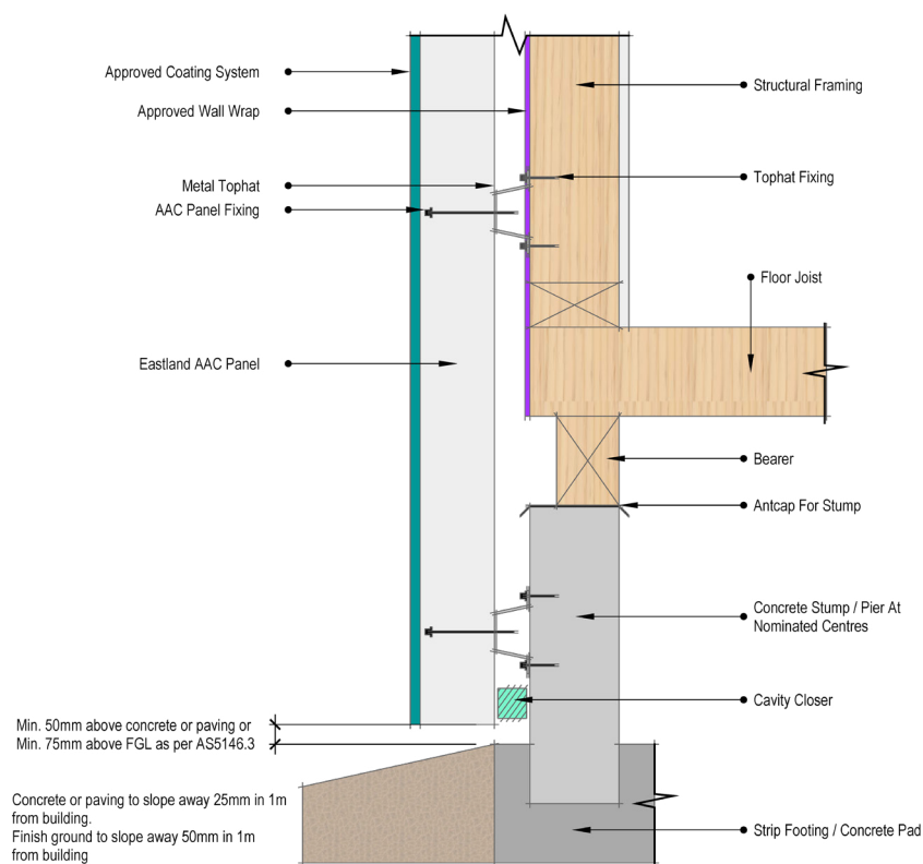
Panels Overhanging Subfloor between Stumps
