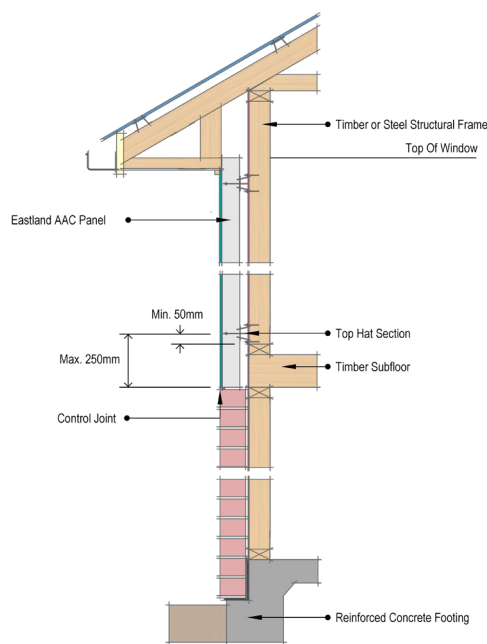
Two Storey Additions - typical section with brick veneer below
