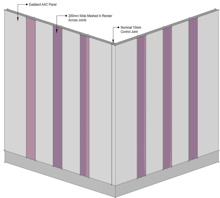
Vertical Control Joint at Building Corners
