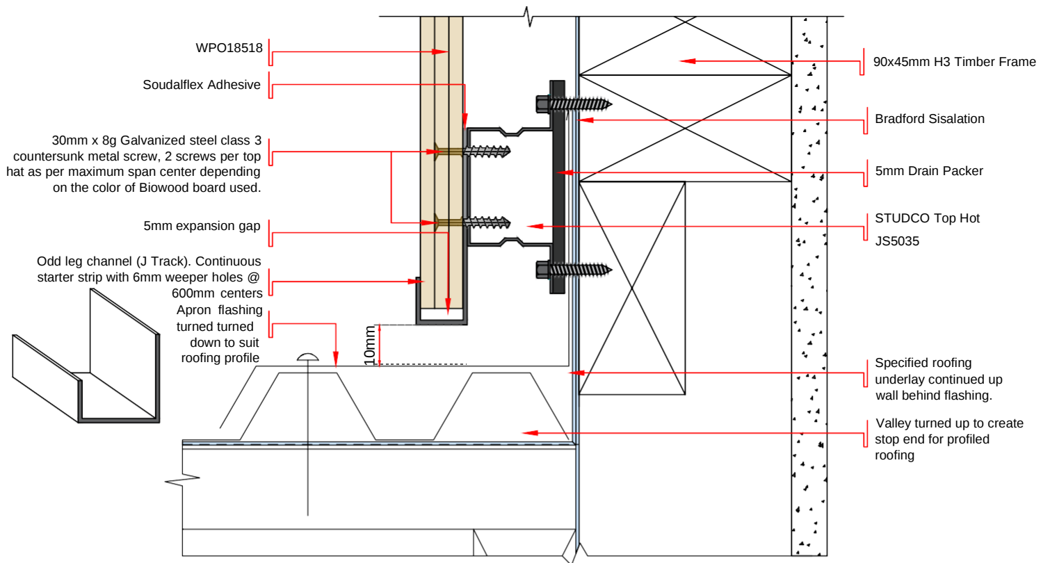
DWG - 10 SECTION VIEW OF PARALLEL APRON DETAIL OF VERTICAL LAID BIOWOOD CLADDING - WPO18518
