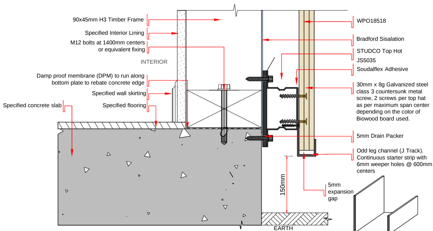
DWG - 03 SECTION VIEW OF CONCRETE EDGE SLAB EDGE DETAIL OF VERTICAL LAID BIOWOOD CLADDING - WPO18518 SCALE 1:2.5 @ A4
