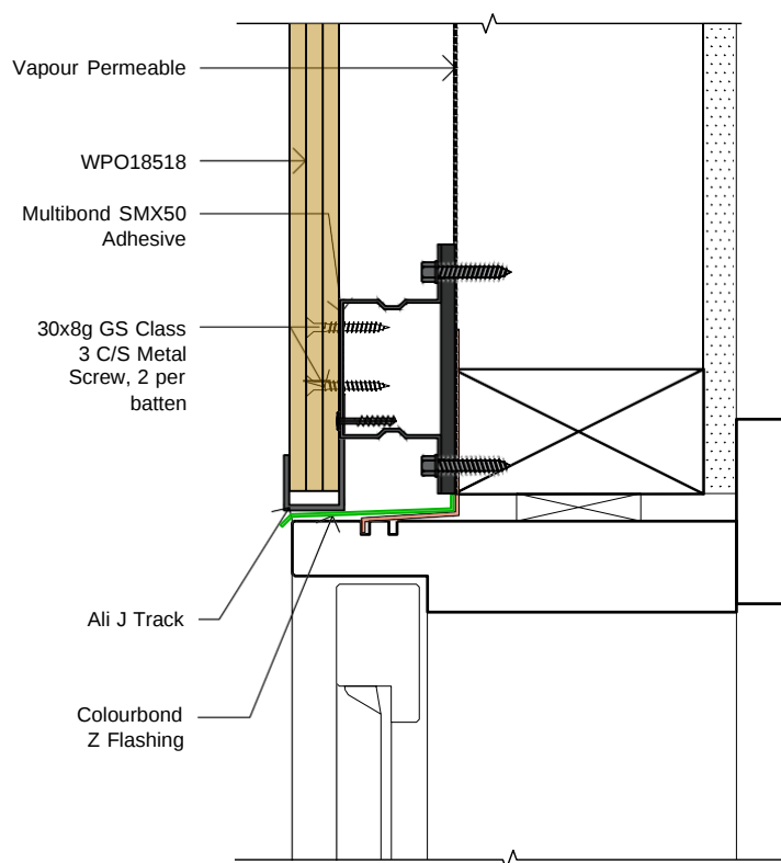
HEADER WINDOW DETAIL W/ J TRACK
