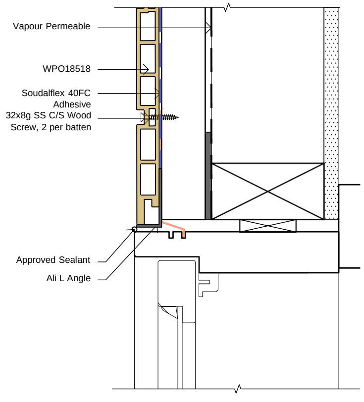
WINDOW JAMB DETAIL W/ ALI L ANGLE
