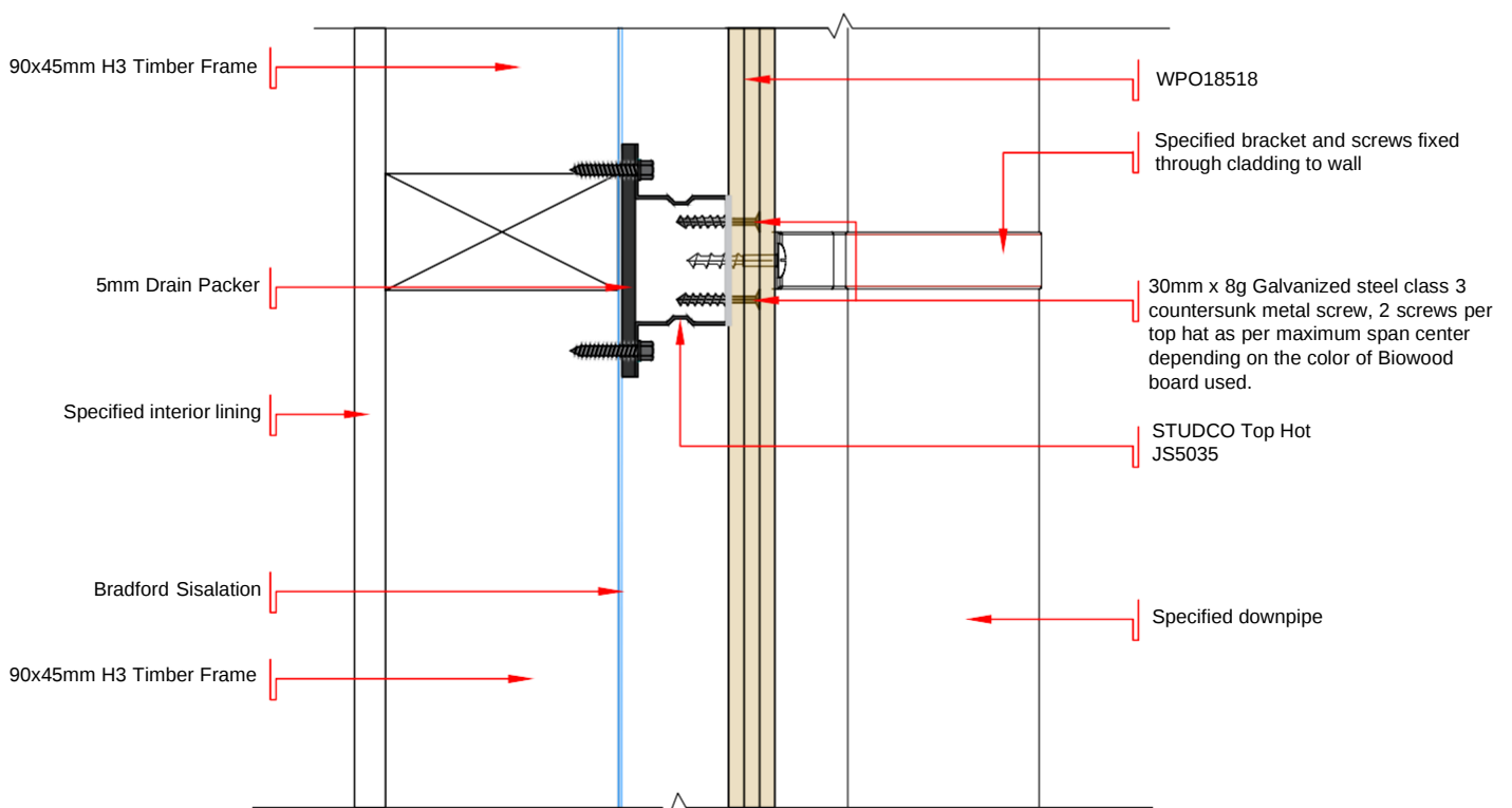
DWG - 13 SECTION VIEW OF DOWNPIPE FIXING DETAIL OF VERTICAL LAID BIOWOOD CLADDING - WPO18518 SCALE 1:3 @ A4
