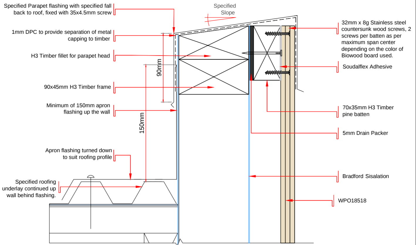
DWG - 12 SECTION VIEW OF PARAPET TO ROOF JUNCTION DETAIL OF VERTICAL LAID BIOWOOD CLADDING - WPO18518 SCALE 1:3 @ A4
