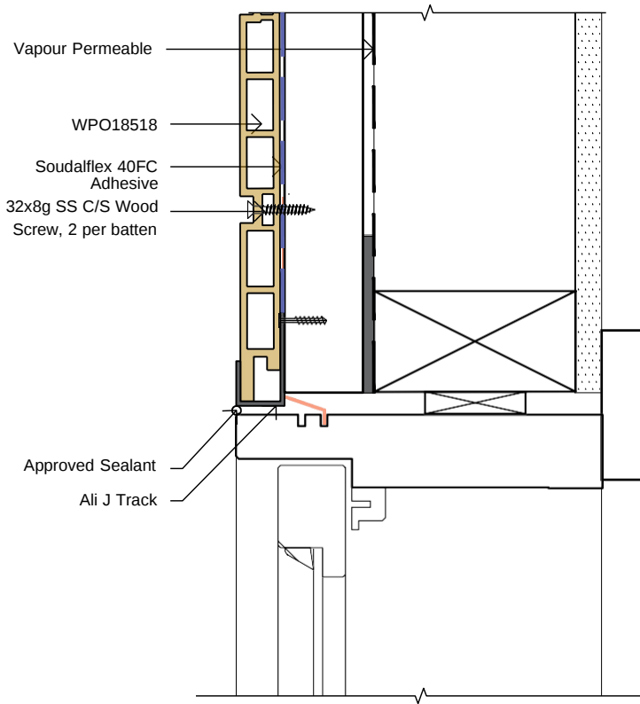
WINDOW JAMB DETAIL W/ J TRACK
