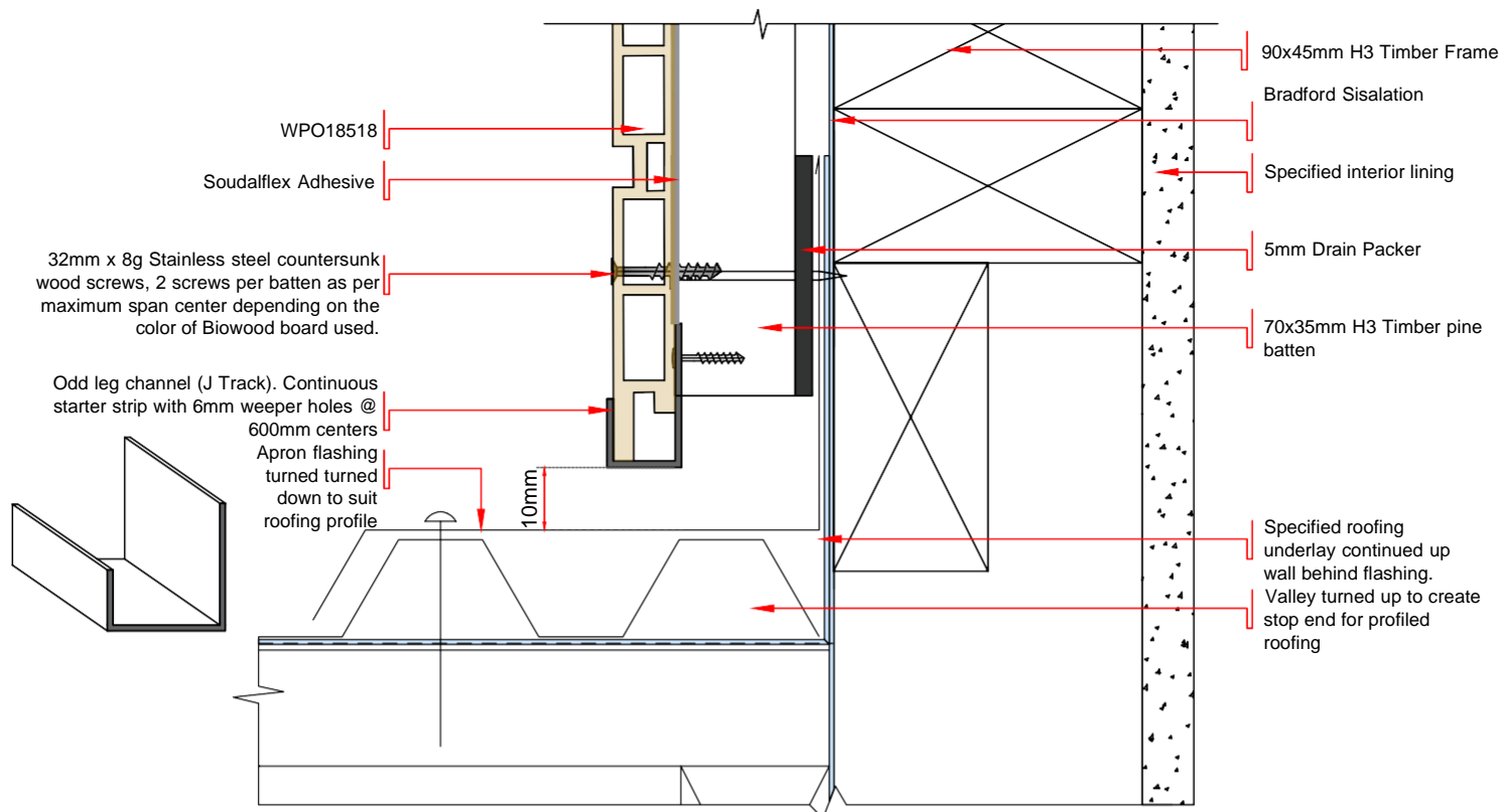
DWG - 10 SECTION VIEW OF PARALLEL APRON DETAIL OF HORIZONTAL LAID BIOWOOD CLADDING - WPO18518
