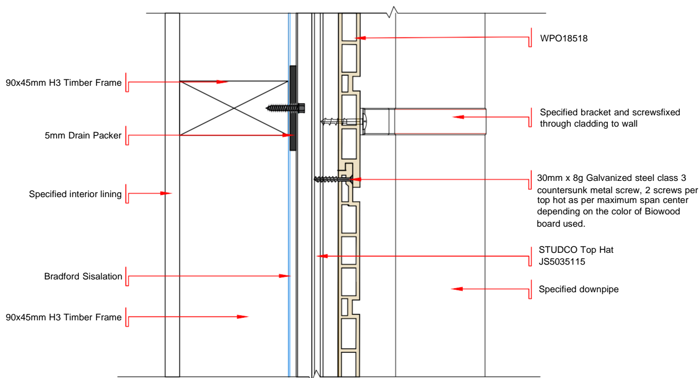
DWG - 13 SECTION VIEW OF DOWNPIPE FIXING DETAIL OF HORIZONTAL LAID BIOWOOD CLADDING - WPO18518 SCALE 1:3 @ A4
