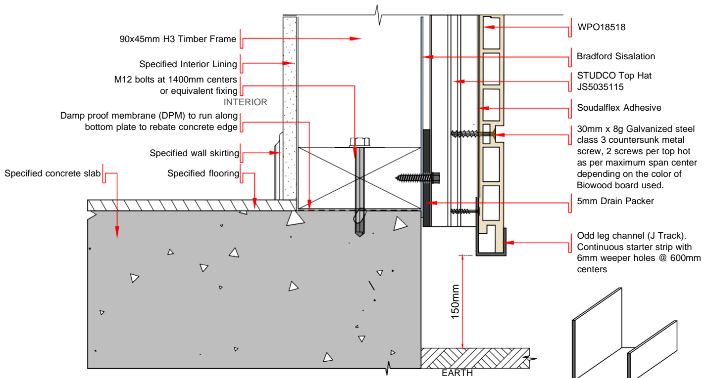
DWG - 03 SECTION VIEW OF CONCRETE EDGE SLAB EDGE DETAIL OF HORIZONTAL LAID BIOWOOD CLADDING - WPO18518 SCALE 1:2.5 @ A4
