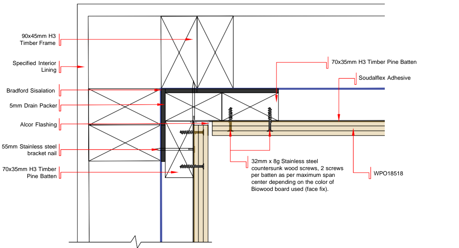
DWG - 05 PLAN VIEW OF INTERNAL CORNER DETAIL OF HORIZONTAL LAID BIOWOOD CLADDING - WPO18518 SCALE 1:3 @ A4
