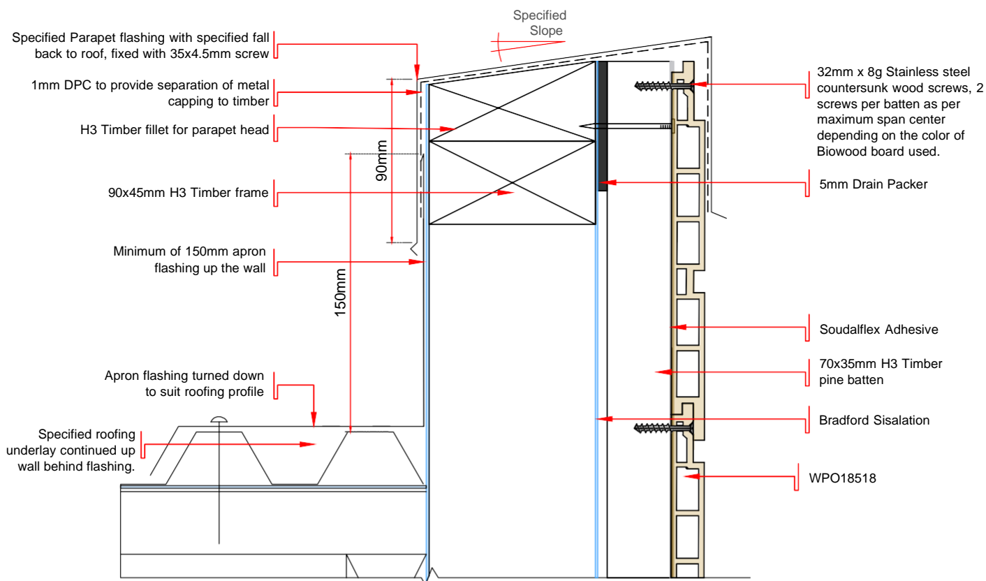
DWG - 12 SECTION VIEW OF PARAPET TO ROOF JUNCTION DETAIL OF HORIZONTAL LAID BIOWOOD CLADDING - WPO18518 SCALE 1:3 @ A4
