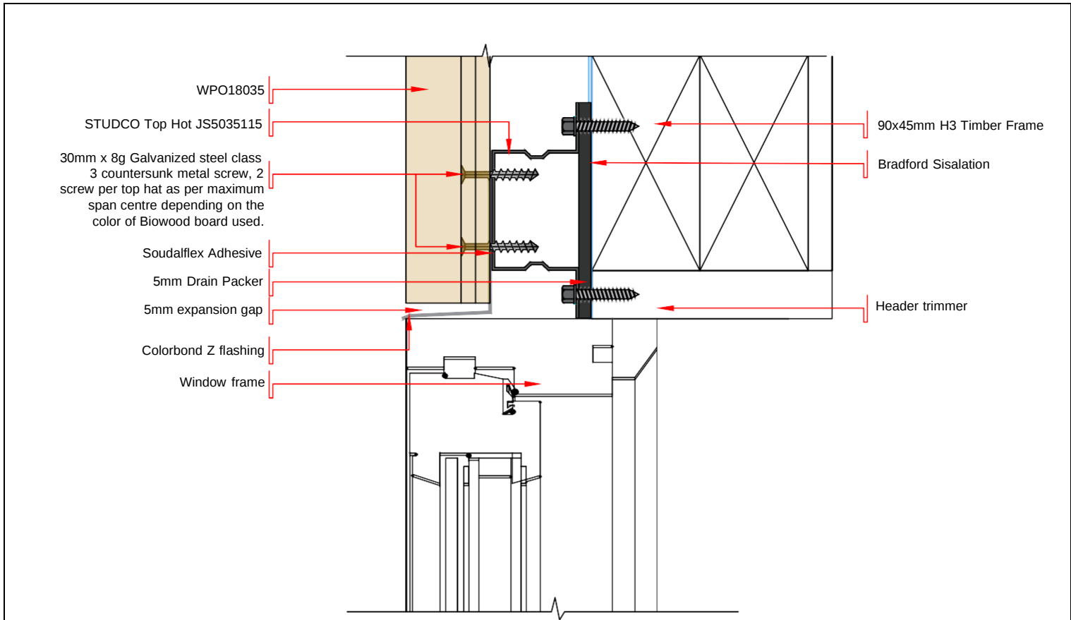
DWG - 06 SECTION VIEW OF WINDOW HEAD DETAIL OF VERTICAL LAID BIOWOOD CLADDING - WPO18035 SCALE 1:2.2 @ A4
