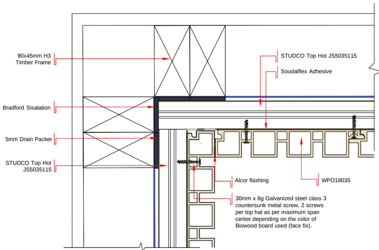
DWG - 05 PLAN VIEW OF INTERNAL CORNER DETAIL OF VERTICAL LAID BIOWOOD CLADDING - WPO18035
