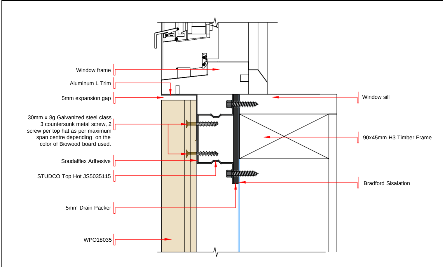
DWG - 07 SECTION VIEW OF WINDOW SILL DETAIL OF VERTICAL LAID BIOWOOD CLADDING - WPO18035 SCALE 1:2.2 @ A4
