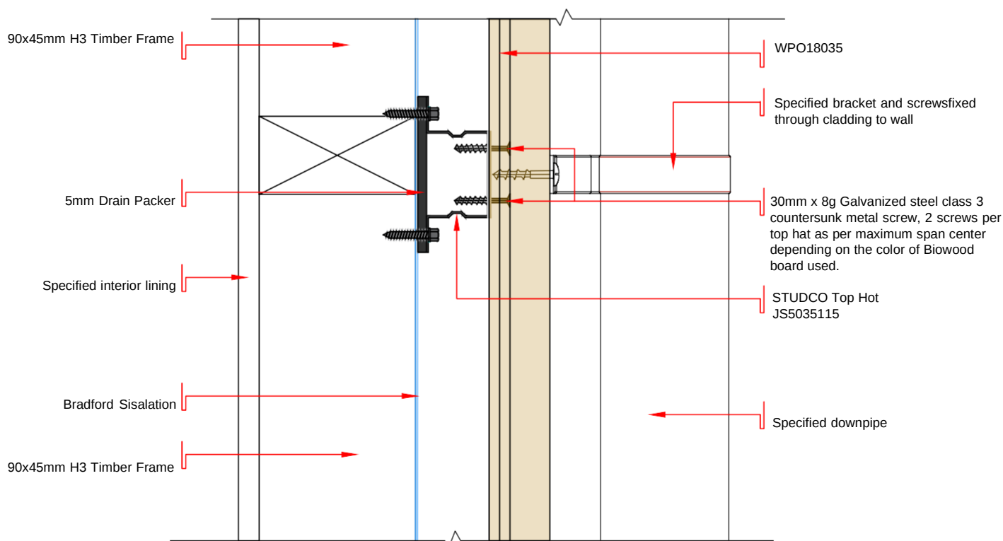
DWG - 13 SECTION VIEW OF DOWNPIPE FIXING DETAIL OF VERTICAL LAID BIOWOOD CLADDING - WPO18035 SCALE 1:3 @ A4
