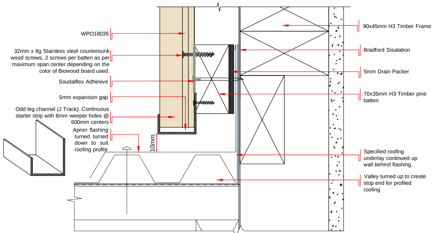
DWG - 10 SECTION VIEW OF PARALLEL APRON DETAIL OF VERTICAL LAID BIOWOOD CLADDING - WPO18035
