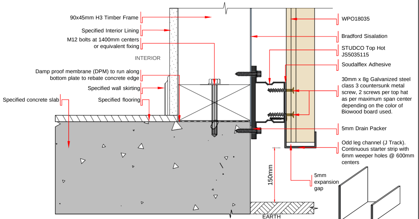
DWG - 03 SECTION VIEW OF CONCRETE EDGE SLAB EDGE DETAIL OF VERTICAL LAID BIOWOOD CLADDING - WPO18035 SCALE 1:2.5 @ A4
