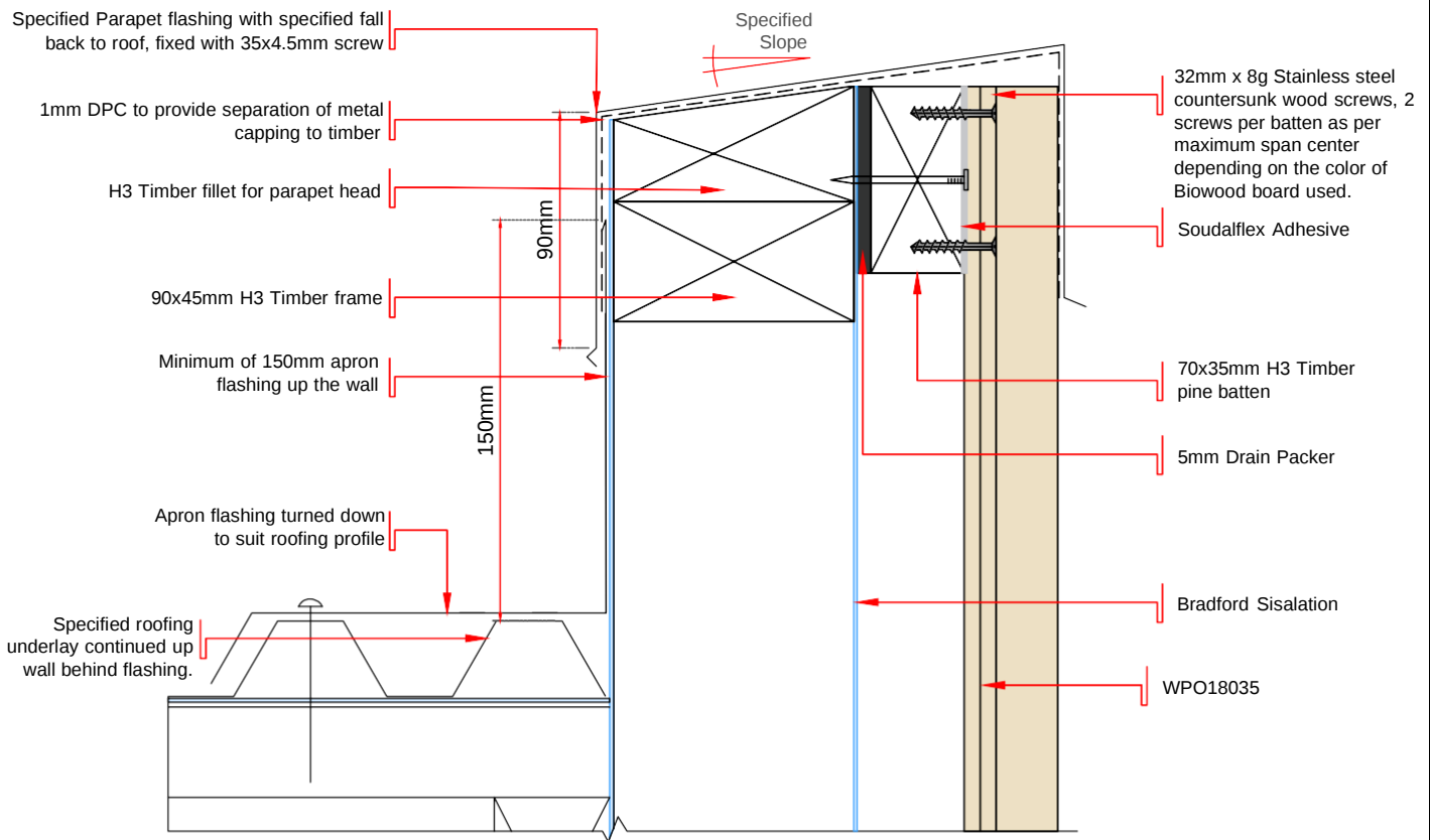
DWG - 12 SECTION VIEW OF PARAPET TO ROOF JUNCTION DETAIL OF VERTICAL LAID BIOWOOD CLADDING - WPO18035 SCALE 1:3 @ A4
