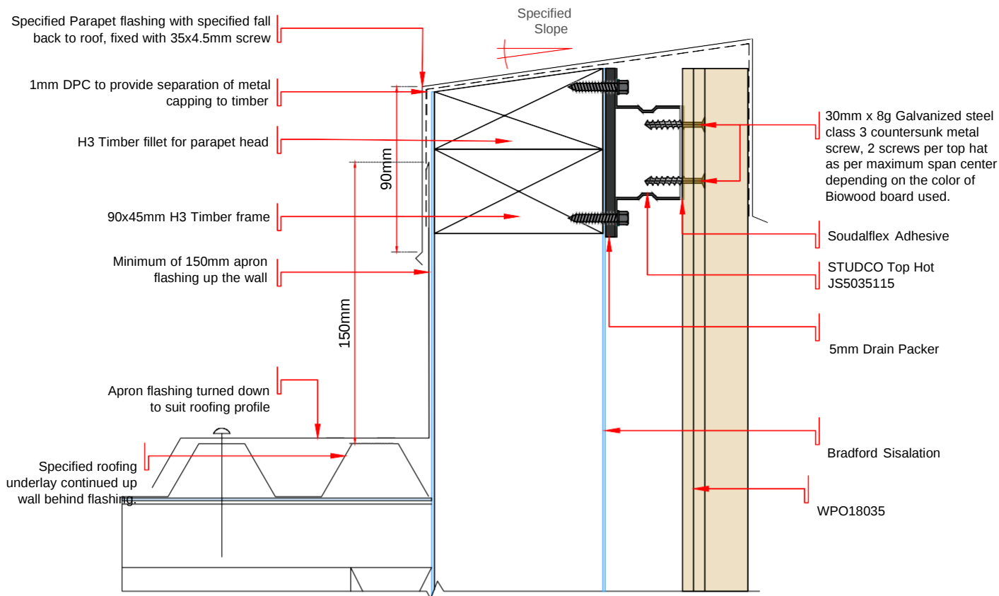
DWG - 12 SECTION VIEW OF PARAPET TO ROOF JUNCTION DETAIL OF VERTICAL LAID BIOWOOD CLADDING - WPO18035 SCALE 1:3 @ A4
