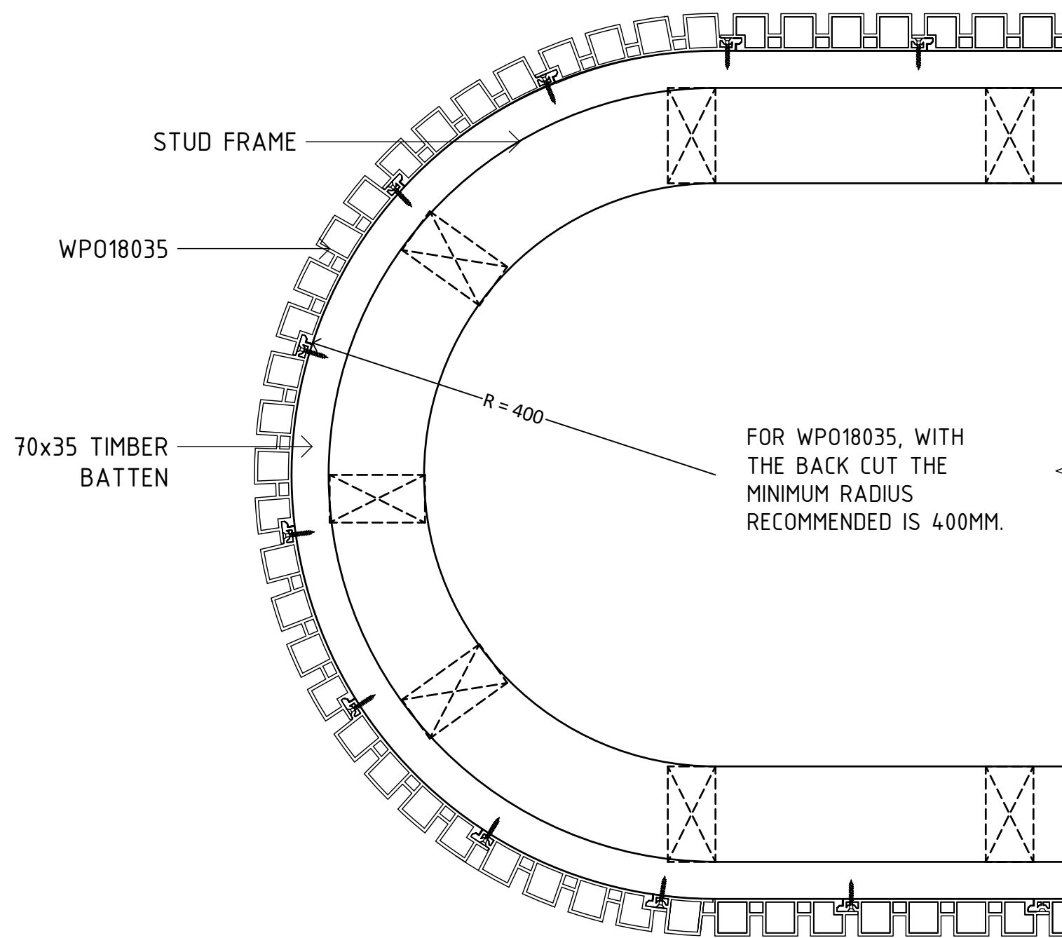
WP018035 VERTICAL CURVED WALL DETAIL SCALE 1:5
