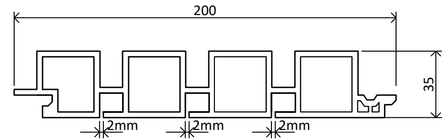
WP018035 BACK CUT DETAIL
