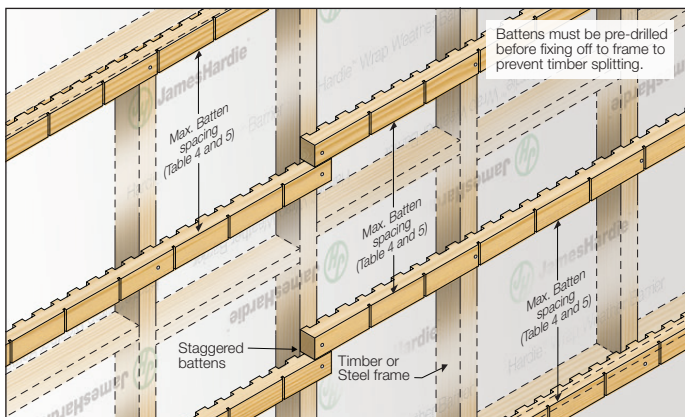
FIGURE 15 ON-STUD STAGGERED JOINTING OF BATTENS
