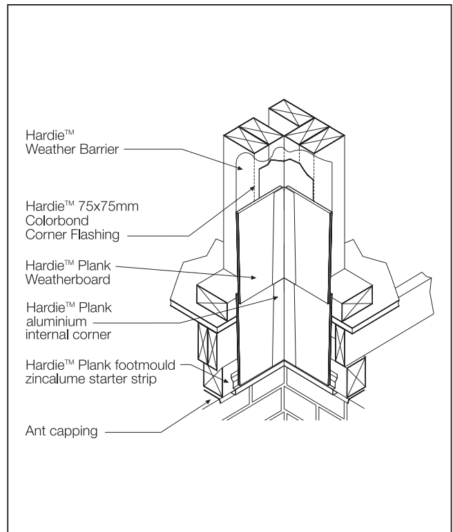
FIGURE 30 INTERNAL CORNER OPTION 3
