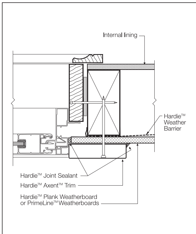
FIGURE 33 WINDOW JAMB DETAIL
