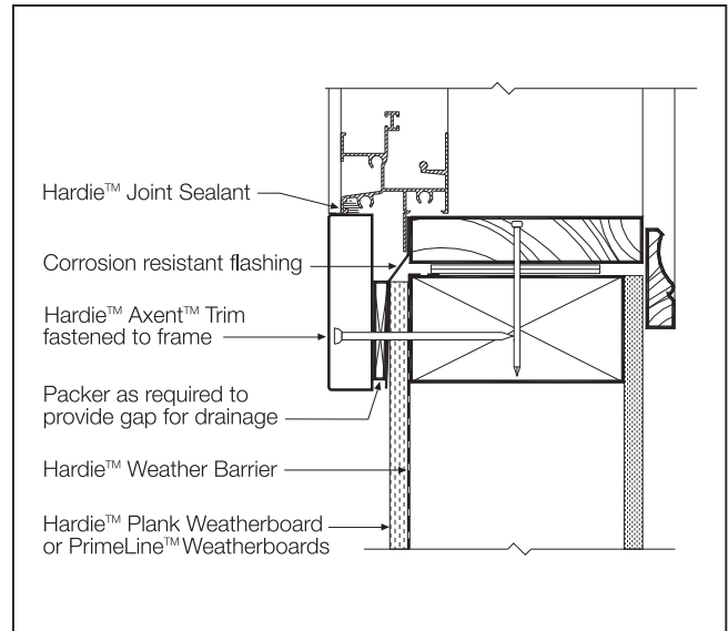
FIGURE 34 WINDOW SILL DETAIL
