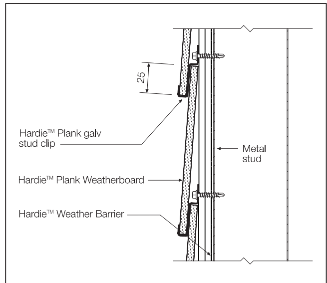
FIGURE 23 FIXING HARDIE™ PLANK STUD CLIPS
