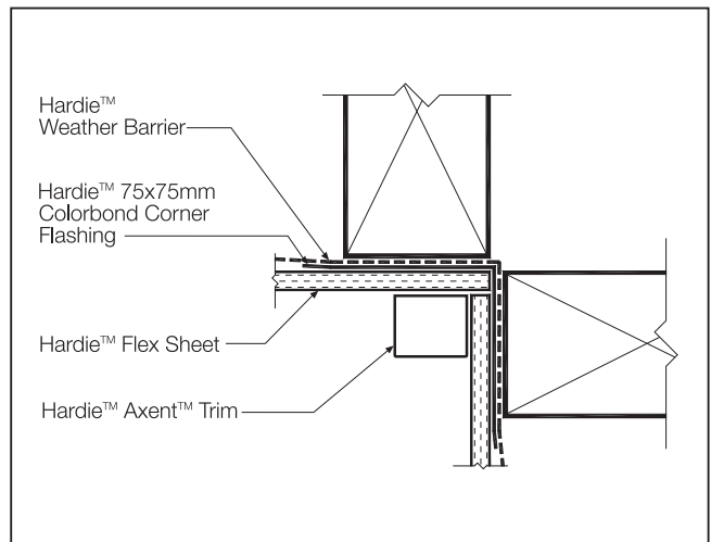
FIGURE 10 INTERNAL TRIM CORNER
