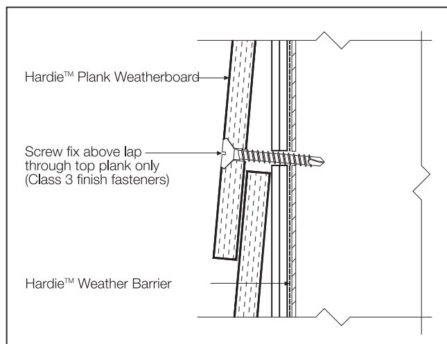
FIGURE 22 SCREW FIXING TO STEEL FRAME
