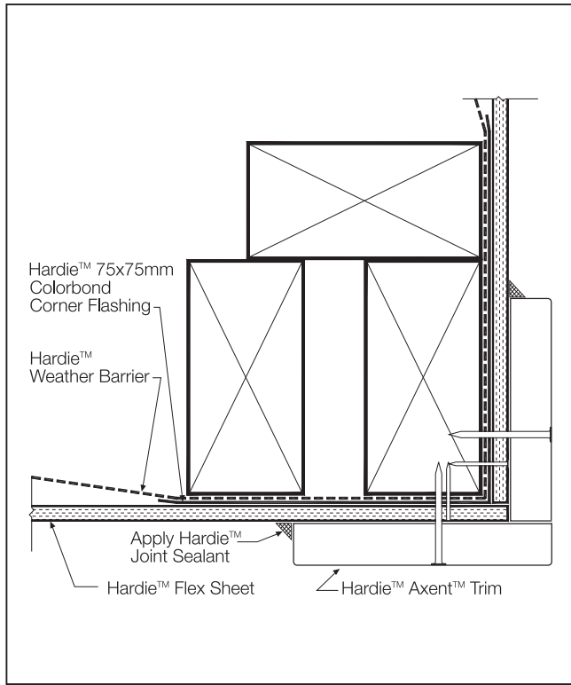
FIGURE 11 HARDIE™ AXENT™ TRIM EXTERNAL CORNER
