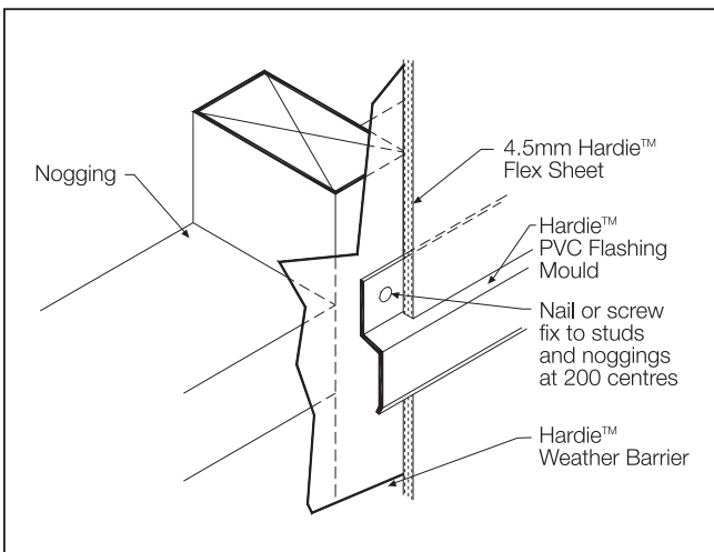
FIGURE 8 DRIP STRIP JOINT
