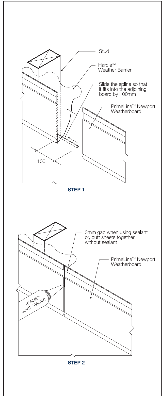
FIGURE 20 OFF-STUD JOINTING
