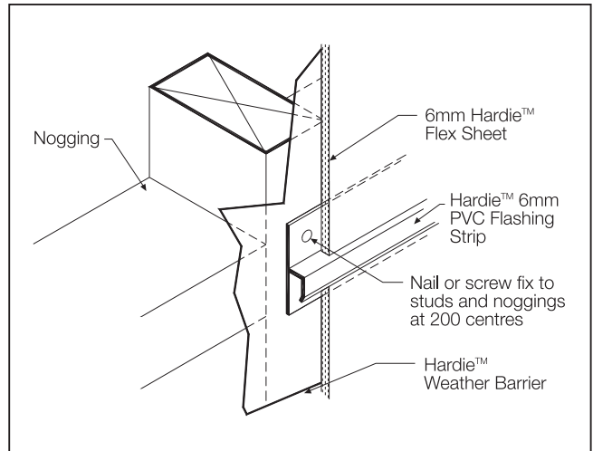
FIGURE 9 HORIZONTAL FLASHING MOULD
