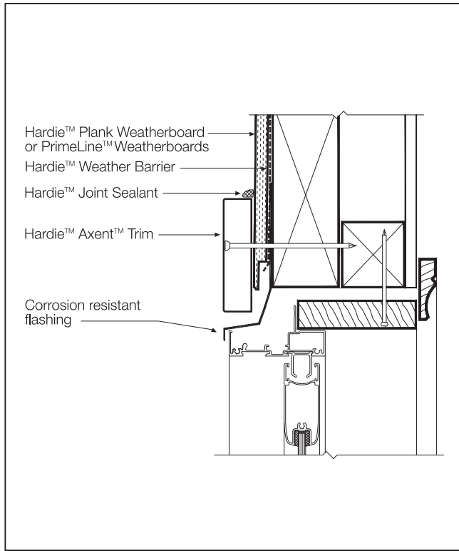
FIGURE 32 WINDOW HEAD DETAIL
