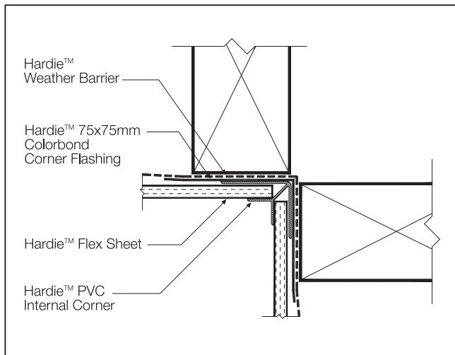
FIGURE 12 PVC INTERNAL CORNER
