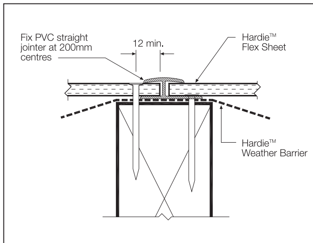
FIGURE 7 PVC STRAIGHT JOINTER
