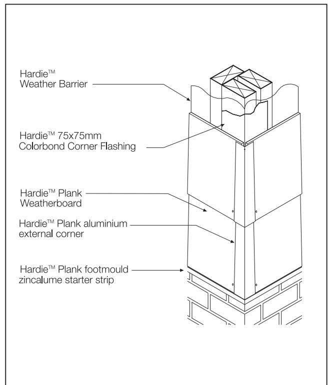
FIGURE 31 EXTERNAL CORNER OPTION 3
