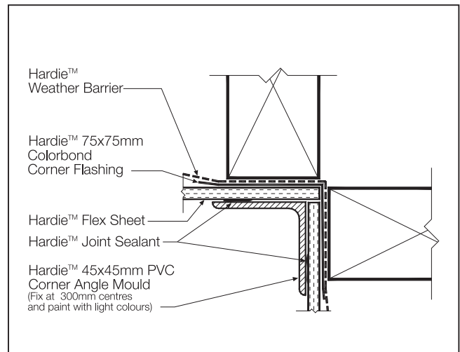
FIGURE 14 PVC CORNER ANGLE MOULD
