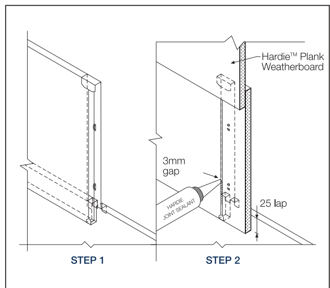
FIGURE 24 FITTING METAL SOAKER
