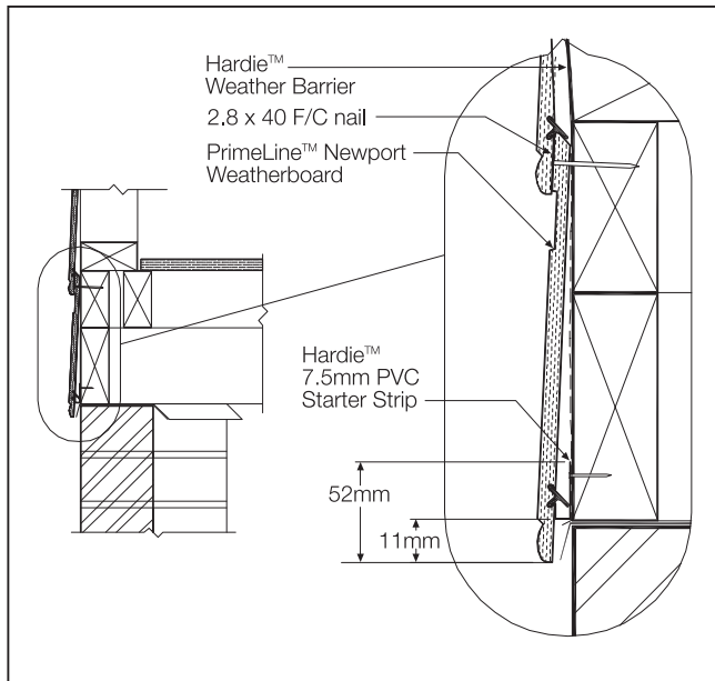
FIGURE 19 INSTALLING FIRST PRIMELINE™ NEWPORT WEATHERBOARD
