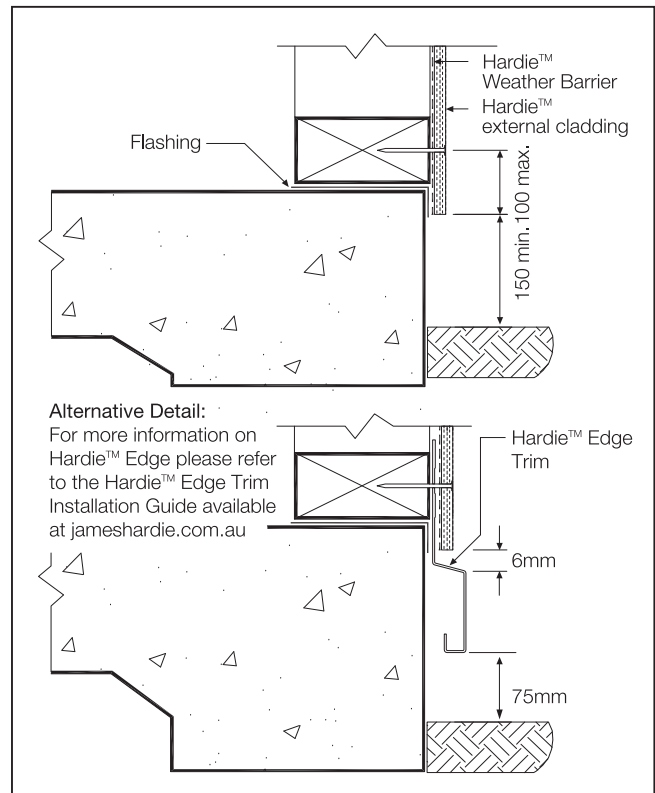
FIGURE 4 TYPICAL DETAIL AT GROUND LEVEL
