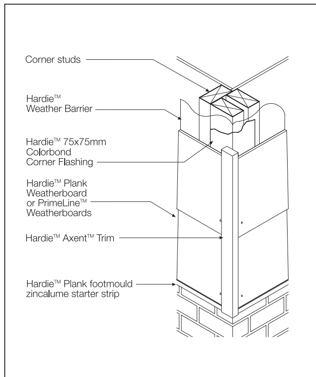
FIGURE 29 EXTERNAL CORNER OPTION 2
