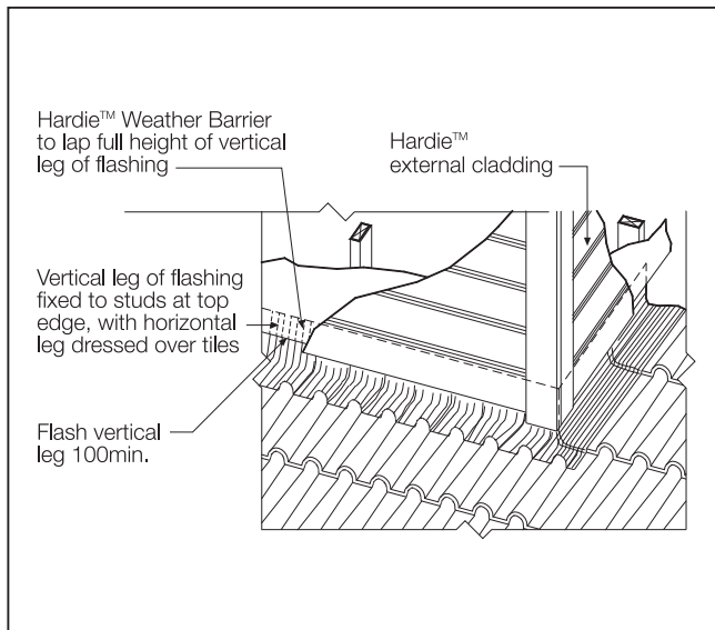
FIGURE 3 SARKING REQUIREMENT FOR EXPOSED CONDITIONS
