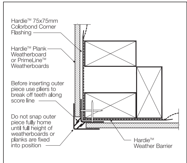
FIGURE 27 EXTERNAL CORNER OPTION 1
