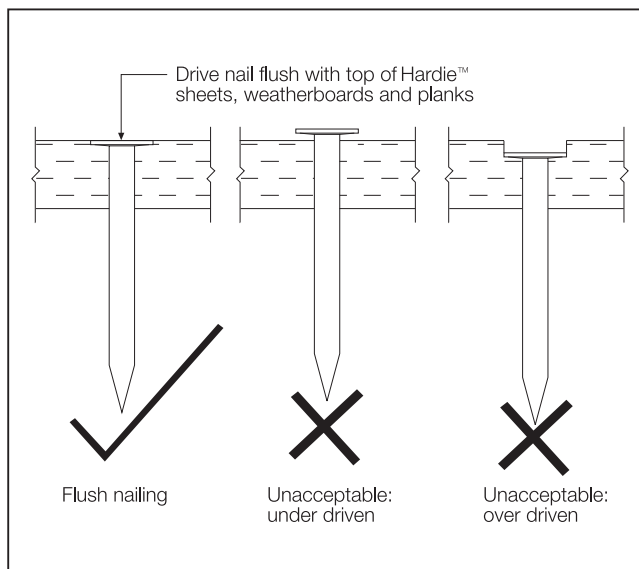
FIGURE 1 NAIL FASTENER DEPTH
