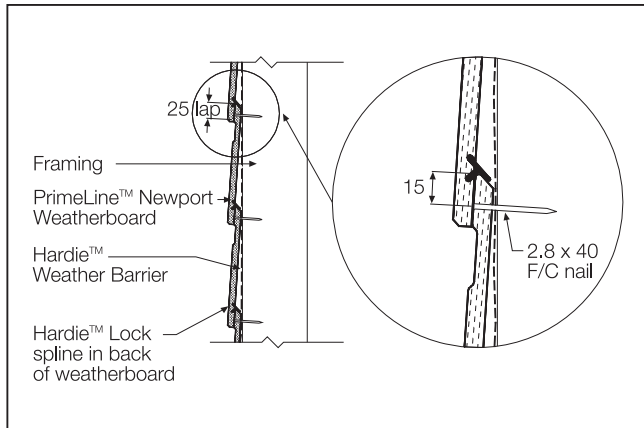
FIGURE 18 NAIL SPACING FOR PRIMELINE™ NEWPORT WEATHERBOARDS
