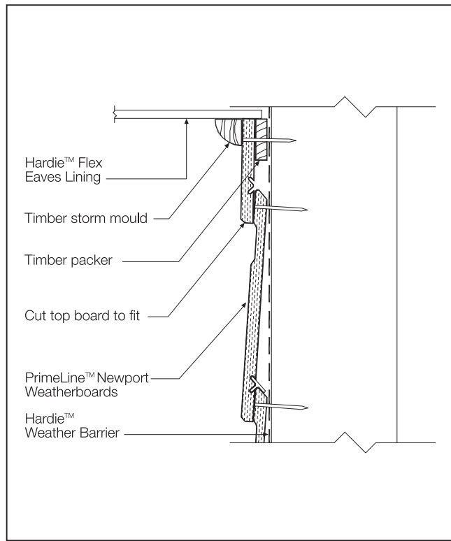
FIGURE 36 DETAIL AT EAVES
