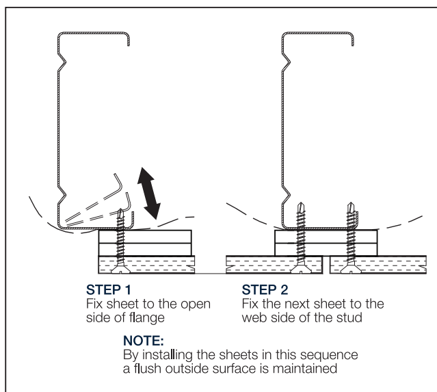
FIGURE 2 SCREW FASTENING
