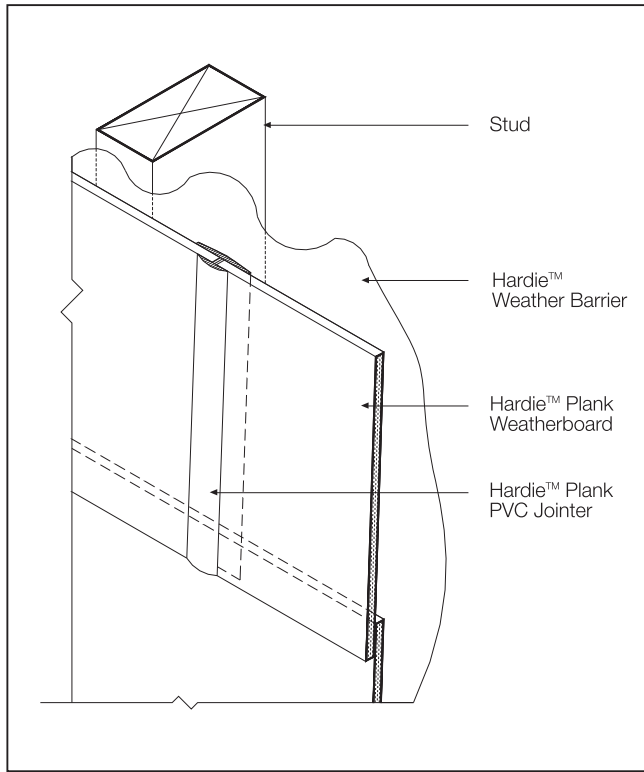
FIGURE 25 PVC JOINTING STRIP
