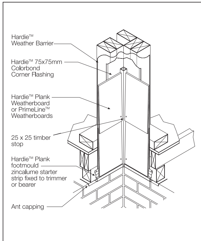
FIGURE 28 INTERNAL CORNER OPTION 2
