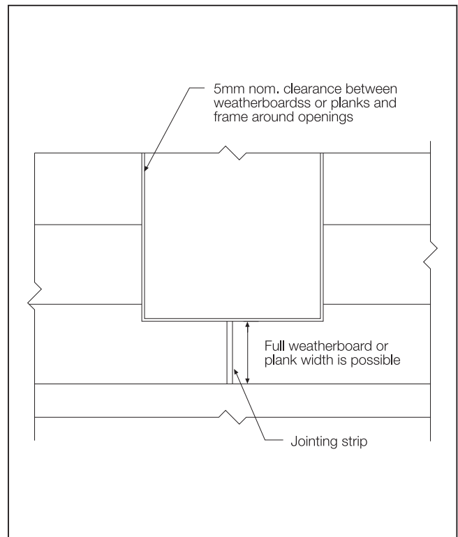
FIGURE 35 CUTTING AROUND OPENINGS
