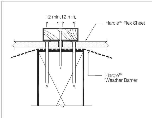
FIGURE 6 TIMBER BATTEN JOINT
