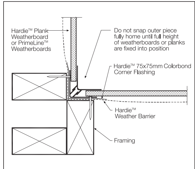
FIGURE 26 INTERNAL CORNER OPTION 1
