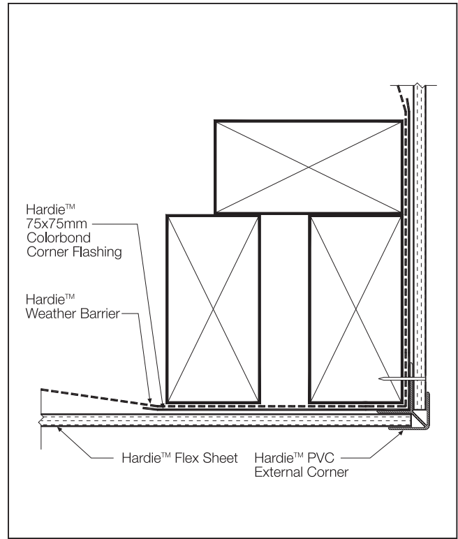
FIGURE 13 PVC EXTERNAL CORNER
