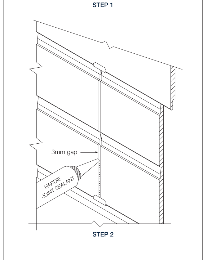
FIGURE 17 UNICLIP ACCESSORY FOR PRIMELINE™ HERITAGE AND CHAMFER WEATHERBOARDS OFF-STUD JOINTING
