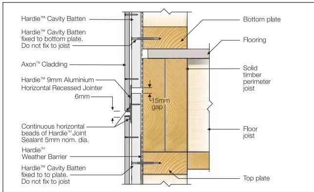
FIGURE 17 FLOOR LEVEL JUNCTION - HORIZONTAL RECESSED JOINTER
