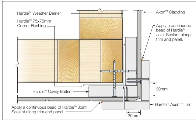
FIGURE 23 TRIM CORNER OPTION - CAVITY BATTEN
