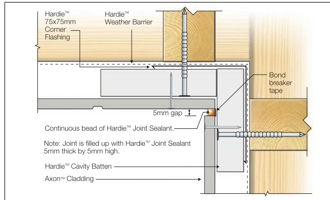
FIGURE 25 SEALANT FILL OPTION - CAVITY BATTEN
