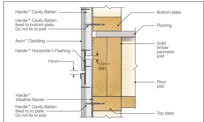
FIGURE 18 FLOOR LEVEL JUNCTION - HORIZONTAL H FLASHING
