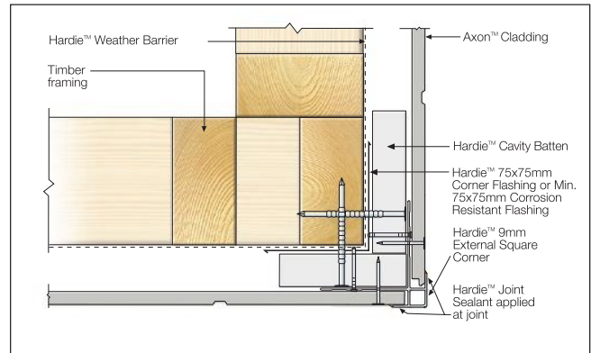
FIGURE 22 ALUMINIUM BOX CORNER OPTION - CAVITY BATTEN
