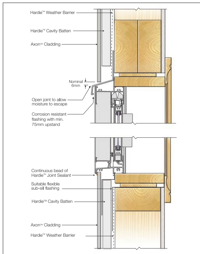
FIGURE 27 WINDOW HEAD AND SILL - CAVITY BATTEN
