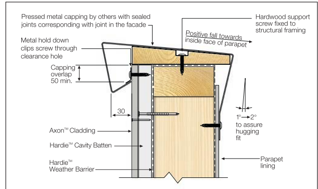
FIGURE 20 PARAPET CAPPING DETAIL
