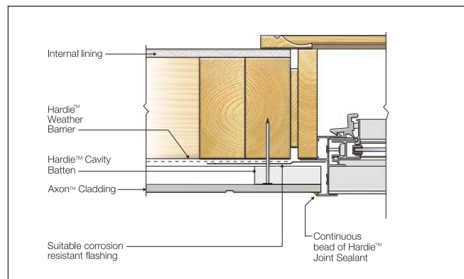
FIGURE 28 WINDOW JAMB - CAVITY BATTEN
