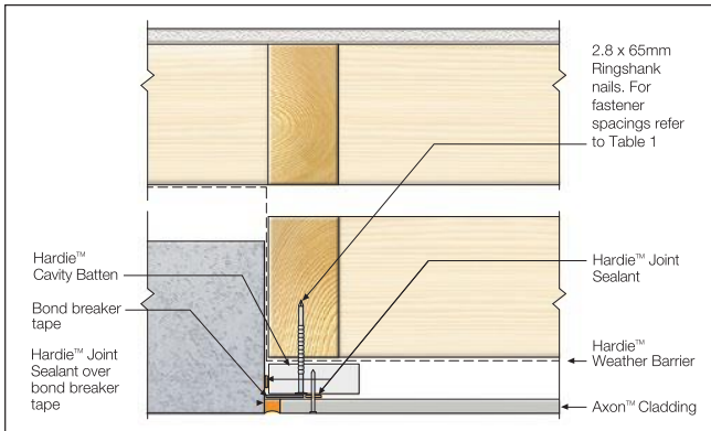
FIGURE 19 ABUTMENT DETAIL
