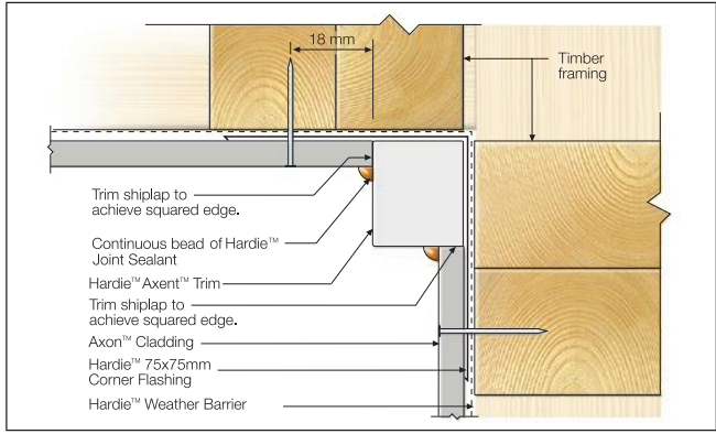
FIGURE 11 TRIM CORNER OPTION
