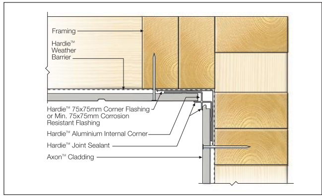
FIGURE 10 ALUMINIUM CORNER DETAIL
