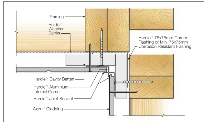
FIGURE 26 ALUMINIUM CORNER DETAIL - CAVITY BATTEN
