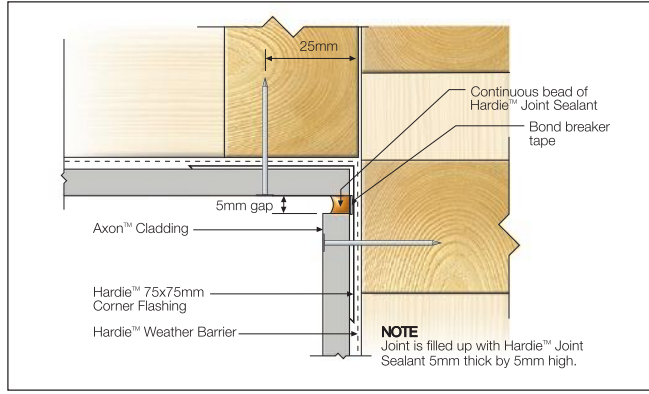
FIGURE 12 SEALANT FILL OPTION
