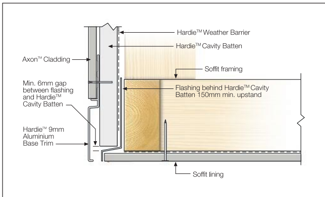
FIGURE 21 FACADE/SOFFIT JUNCTION
