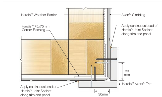
FIGURE 8 TRIM CORNER OPTION
