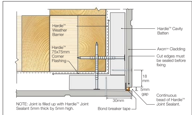
FIGURE 24 SEALANT FILL OPTION - CAVITY BATTEN
